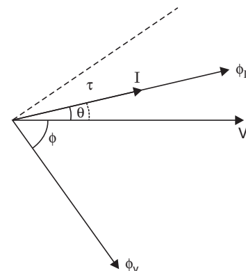
Fig. 14.11 Phasor diagram of a directional relay.
