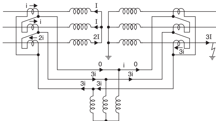
Fig. 14.48 Transformer star/star grounded CT delta connected protection.
