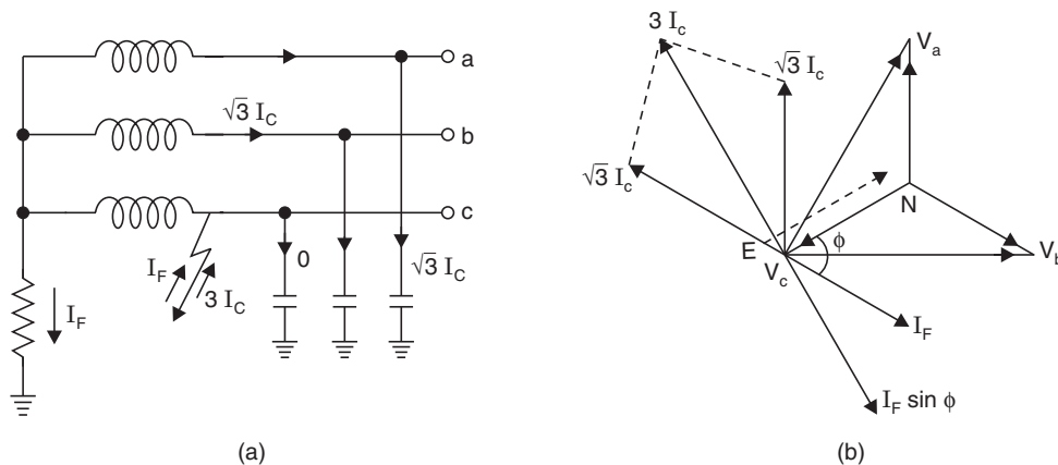
Fig. 11.5 (a) Resistance grounded system, (b) Phasor diagram.
