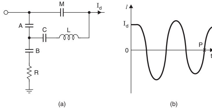
Fig. 5.24 (a) Schematic diagram of a d.c. switch (oscillatory discharge). (b) Current waveform through M .
