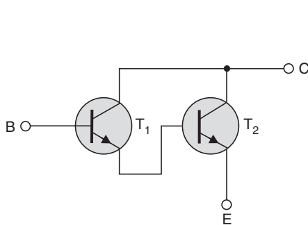
Fig. 14.93 Darlington circuit.
