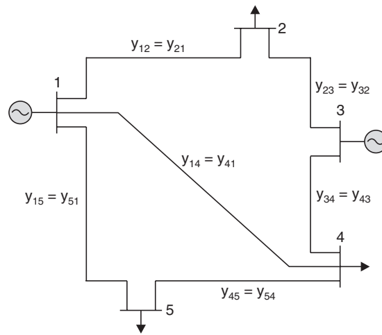
Fig. 18.2 Five-bus system.
