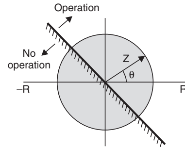
Fig. 14.15 Operating characteristic of an impedance relay with directional unit.
