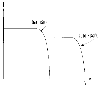
FIGURE 8-15 Effect of temperature on the i-v characteristic. The cell produces less current but greater voltage, with net gain in the power output at cold temperature.
