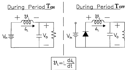
FIGURE 11-7 Charge converter operation during switch on-time and off-time.
