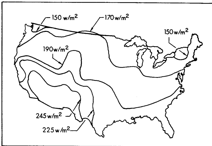
FIGURE 3-16 Yearly 24-hour average solar radiation in watts/m 2 reaching the horizontal surface of the earth. (Source: ProPles in Renewable Energy, DOE/NREL Report No. DE-930000081, August 1994.)
