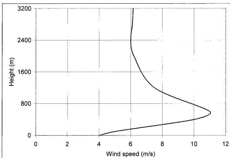
FIGURE 4-16 Wind-speed variations with height measured at Merida airport in Mexico. (Source: Schwartz and Elliott, DOE/NREL Report DE95009202, May 1995.)
