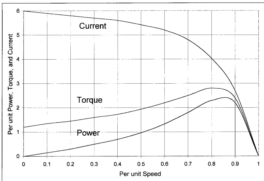
FIGURE 6-11 Induction machine starting and accelerating characteristic.
