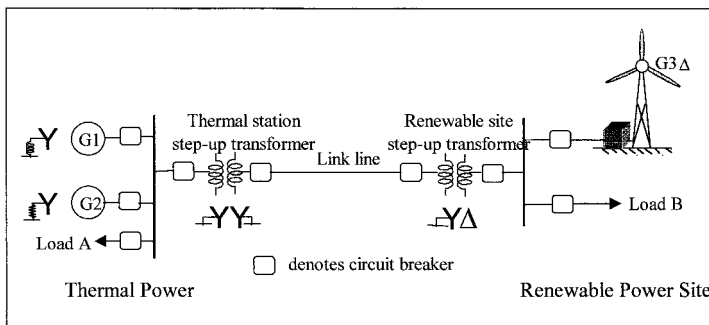
FIGURE 14-2 One-line schematic diagram of grid-connected wind farm.
