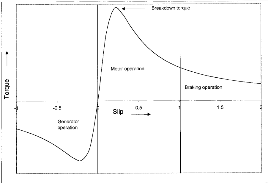
FIGURE 6-9 Torque versus speed characteristic of the induction machine in three operating modes.
