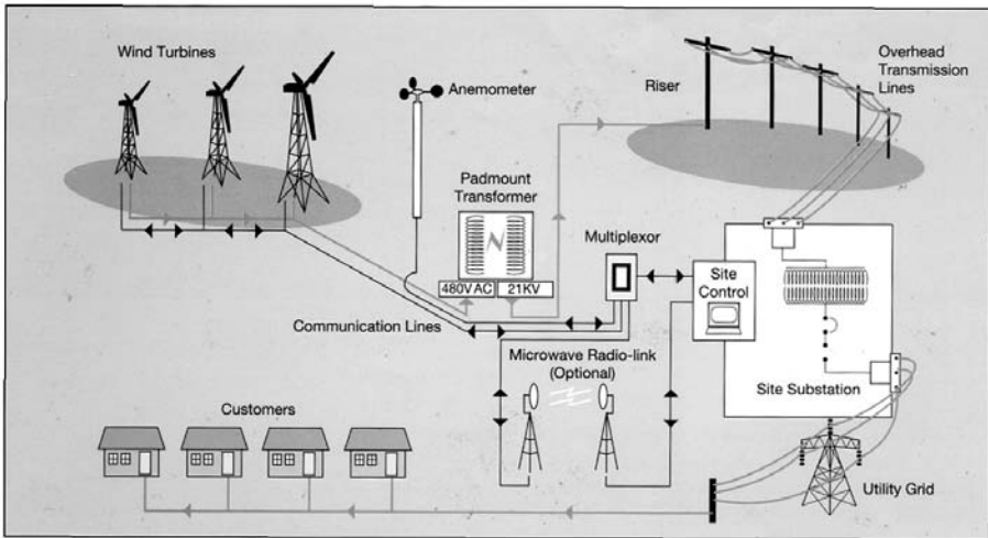
FIGURE 13-4 Electrical component layout of the grid-connected wind power system. (Source: AWEA/IEA/ CADET Technica Brochure, 1995.)
