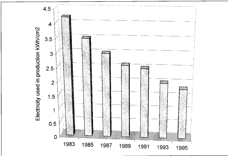
FIGURE 3-6 Energy consumption per \text{cm}^2 of pv cell manufactured. (Source: U.S. Department of Commerce and Dataquest, Inc.)
