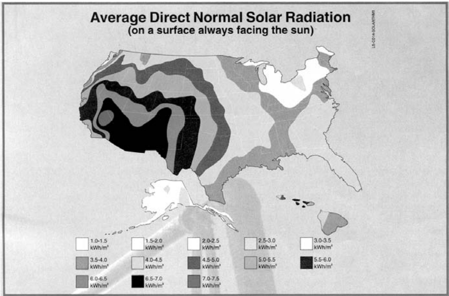
FIGURE 3-18 Yearly 24-hour average solar energy in kWh/m 2 reaching surface always facing the sun at right angel. (Source: A. Anson, ProPles in Renewable Energy, DOE/NREL Report No. DE-930000081, August 1994.)
