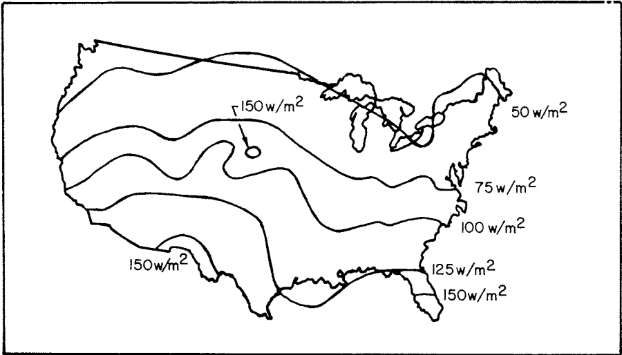
FIGURE 3-17 December 24-hour average solar radiation in watts/m 2 reaching the horizontal surface of the earth. (Source: ProPles in Renewable Energy, DOE/NREL Report No. DE-930000081, August 1994.)
