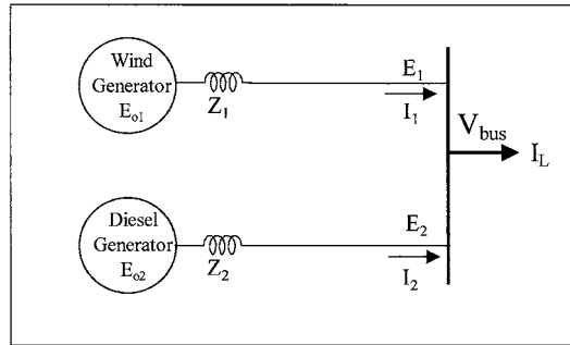
FIGURE 12-14 Thevenin's equivalent model of two sources in hybrid power system.
